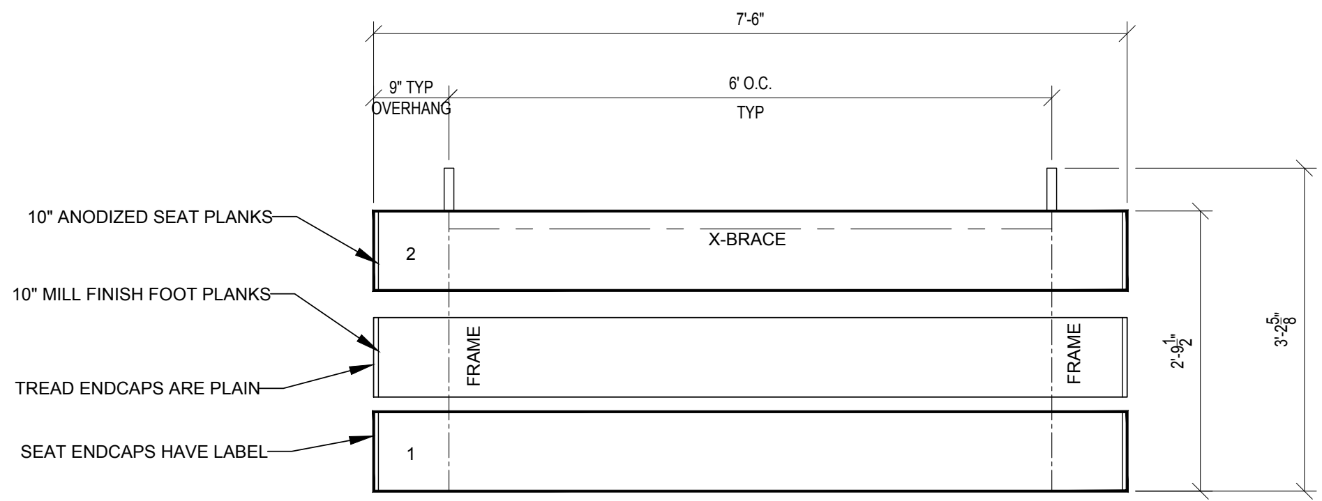
SEATING PLAN SCALE: 3/4" = 1' - 0"
