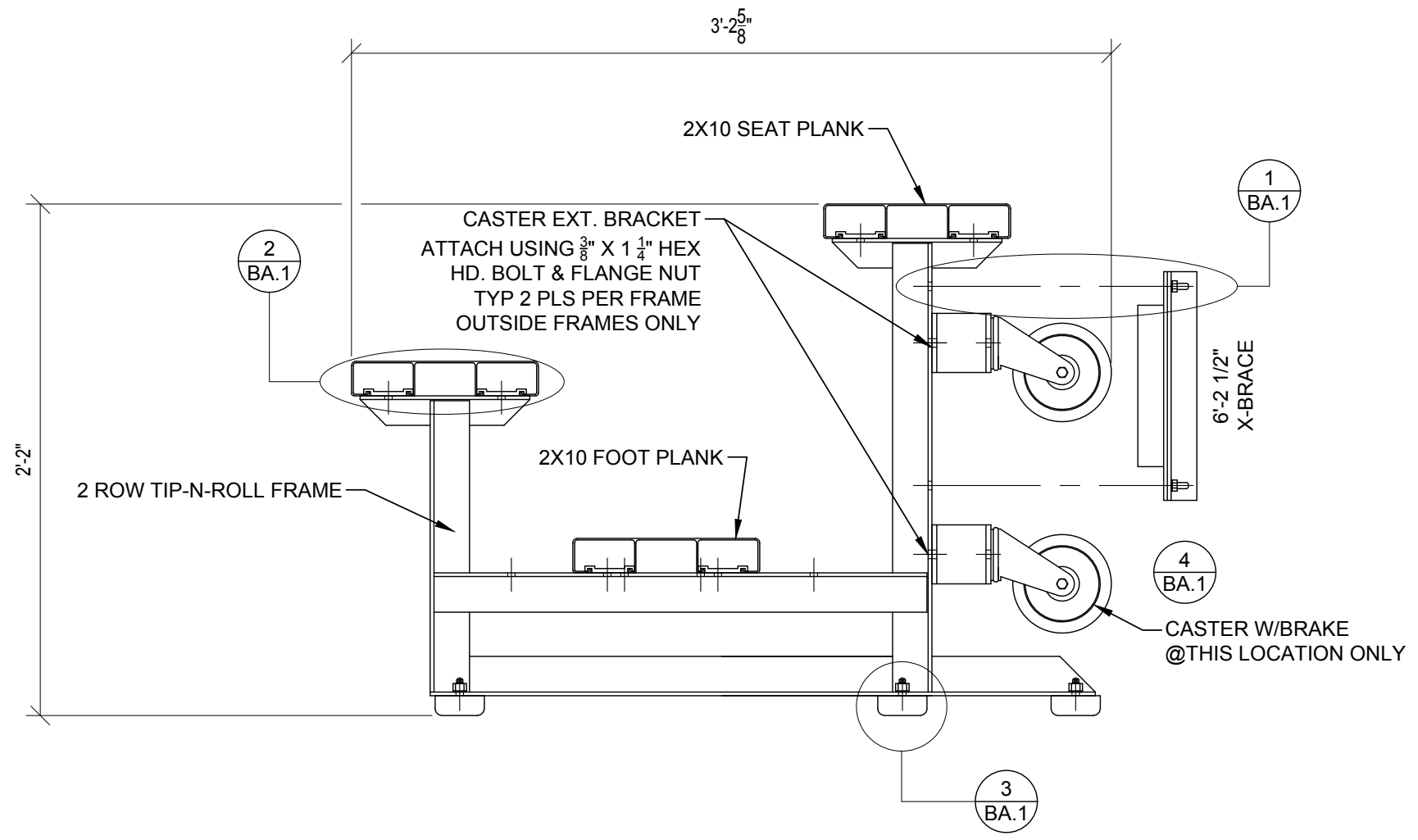
BLEACHER ASSEMBLY ELEVATION
