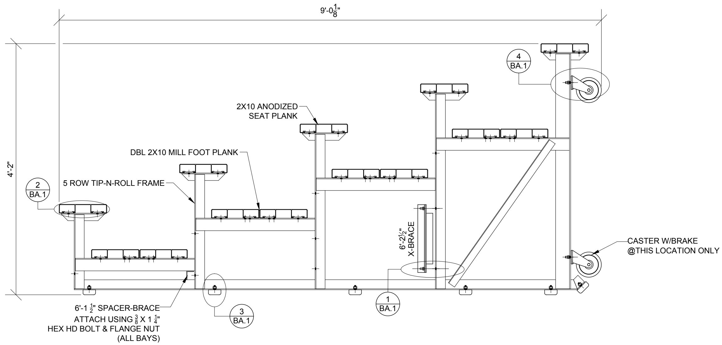
BLEACHER ASSEMBLY ELEVATION SCALE: 1" = 1' - 0"
