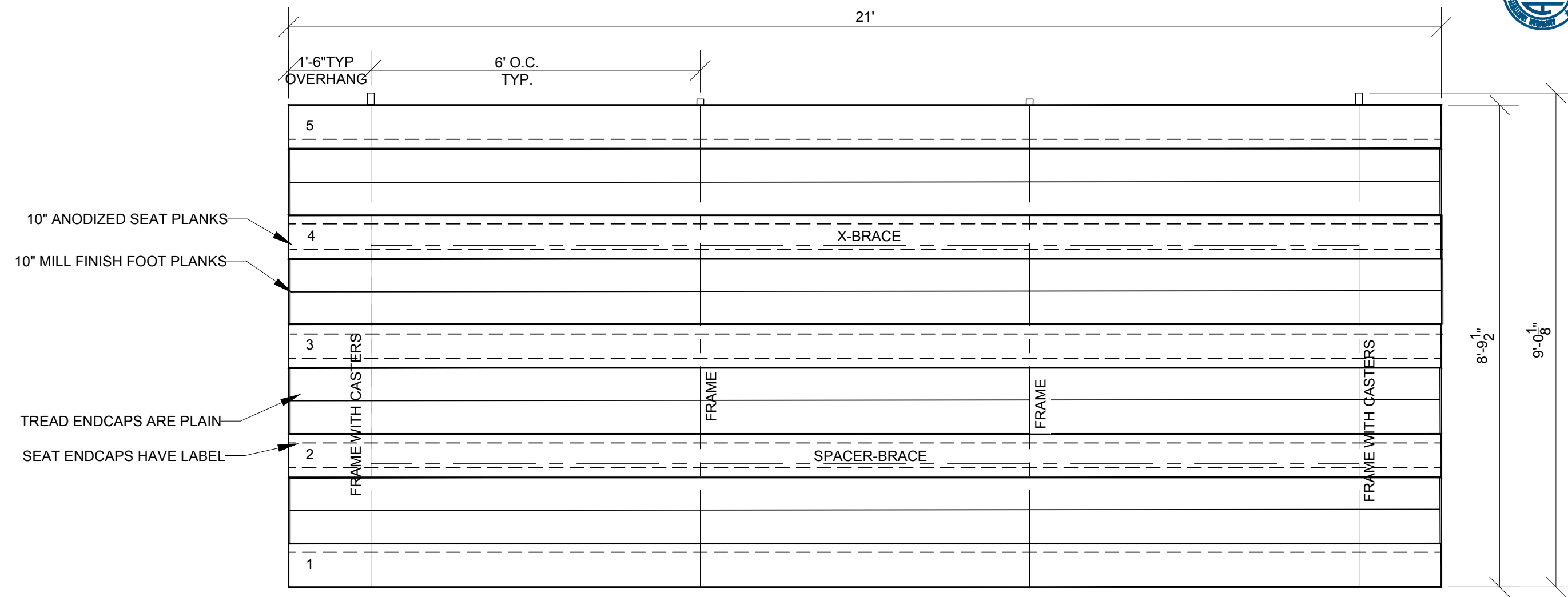
SEATING PLAN SCALE: 1/2" = 1' - 0"
